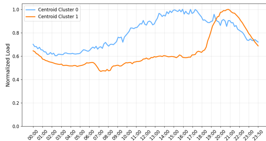
Figure 10. Normalized characteristic curves of transformers.
